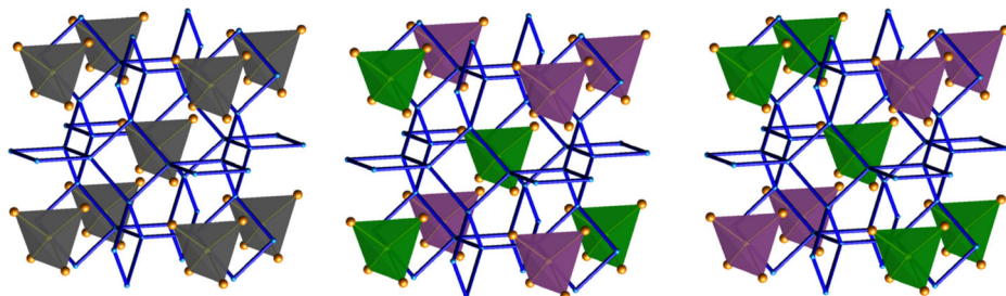
Fig. 18 Representation of magnetic correlations in \text{Fe}_8(\text{BeSiO}_4)_6\text{Se}_2 as a function of temperature. Left - grey tetrahedra represent paramagnetic state; centre - individual tetrahedra have some magnetic correlations (green and purple tetrahedra represent different possible spin orientations in the frustrated arrangement); right - a possible three dimensionally magnetically ordered arrangement of individual tetrahedra
